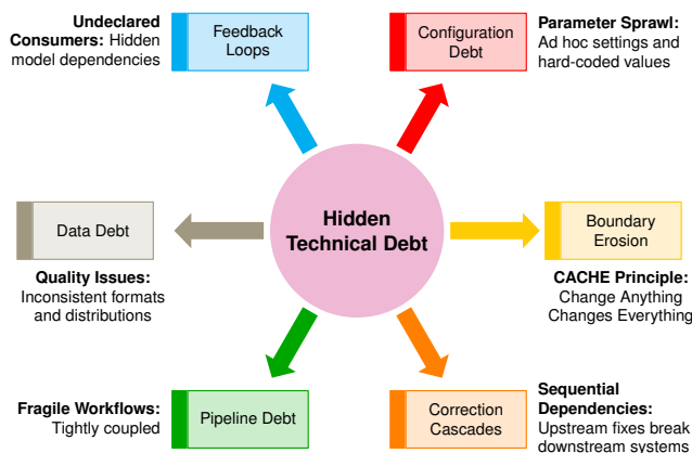
Figure 13.3: ML Technical Debt Taxonomy: Machine learning systems accumulate distinct forms of technical debt that emerge from data dependencies, model interactions, and evolving requirements. This hub-and-spoke diagram illustrates the primary debt patterns: boundary erosion undermines modularity, correction cascades propagate fixes through dependencies, feedback loops create hidden coupling, while data, configuration, and pipeline debt reflect poorly managed artifacts and workflows. Understanding these patterns enables systematic engineering approaches to debt prevention and mitigation.
