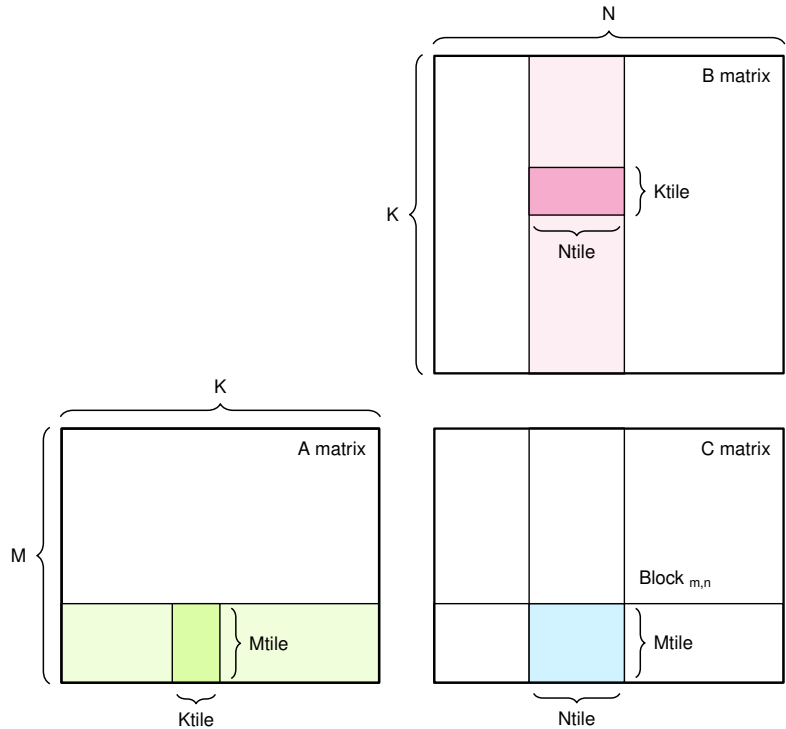
Figure 11.8: Matrix Tiling: Partitioning large matrices into smaller tiles optimizes data reuse and reduces memory access overhead during computation. This technique improves performance on AI accelerators by enabling efficient loading and processing of data in fast memory, minimizing transfers from slower main memory.
