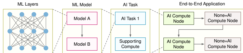
Figure 12.3: Benchmarking Granularity: ML system performance assessment occurs at multiple levels, from end-to-end application metrics to individual model and hardware component efficiency, enabling targeted optimization and bottleneck identification. This hierarchical approach allows practitioners to systematically analyze system performance and prioritize improvements based on specific component limitations.
