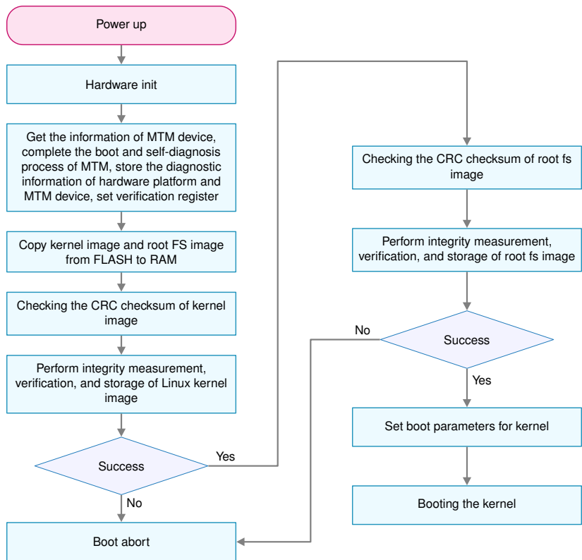
Figure 15.16: Secure Boot Sequence: Embedded systems employ a layered boot process to verify firmware and software integrity, establishing a root of trust before executing machine learning workloads and protecting against pre-runtime attacks. This architecture ensures only authenticated code runs, safeguarding model data and preventing unauthorized model substitution or modification during deployment. Source: (R. V. and A. 2018).
