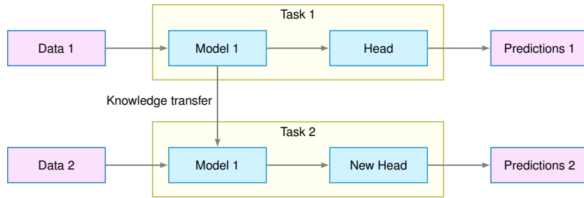
Figure 16.34: Knowledge Transfer: Pre-training on large datasets enables models to learn generalizable features, which can then be fine-tuned for specific target tasks with limited labeled data. This approach mitigates data scarcity and accelerates learning in new domains by leveraging previously acquired knowledge. Source: bhavsar
