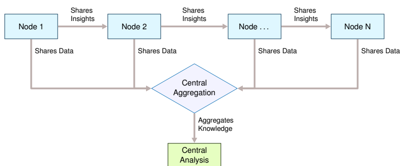
Figure 19.5: Distributed Knowledge Architecture: Autonomous nodes collaboratively process data and share insights via communication networks, enabling scalable and adaptable AI systems through decentralized knowledge aggregation and analysis. This pattern decouples data processing from centralized control, fostering resilience and allowing systems to respond effectively to dynamic environments and distributed data sources.
