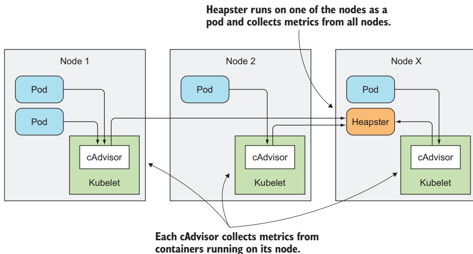
Figure 14.8 The flow of metrics data into Heapster
