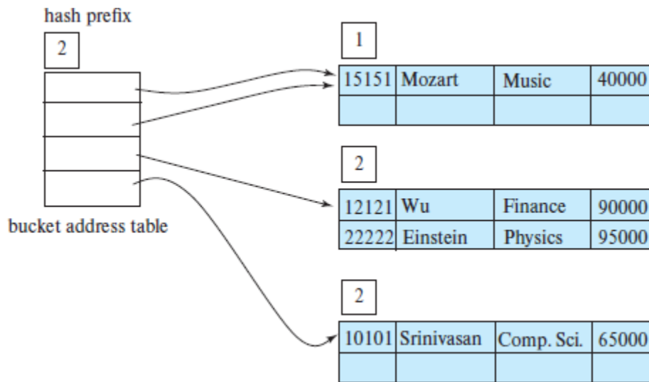
Figure 24.12 Hash structure after four insertions.
