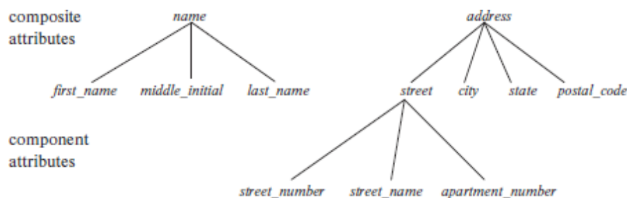
Figure 6.7 Composite attributes instructor name and address .
