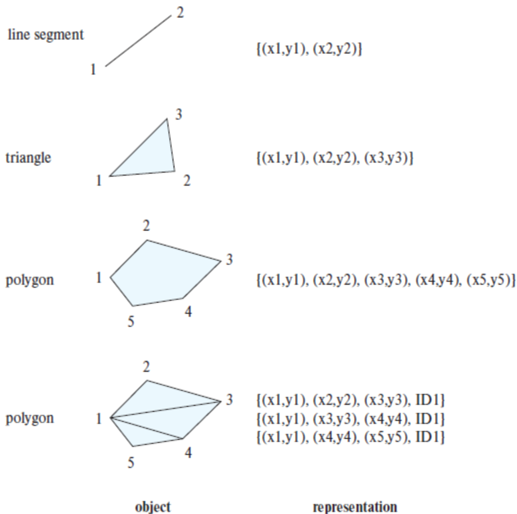
Figure 8.5 Representation of geometric constructs.
