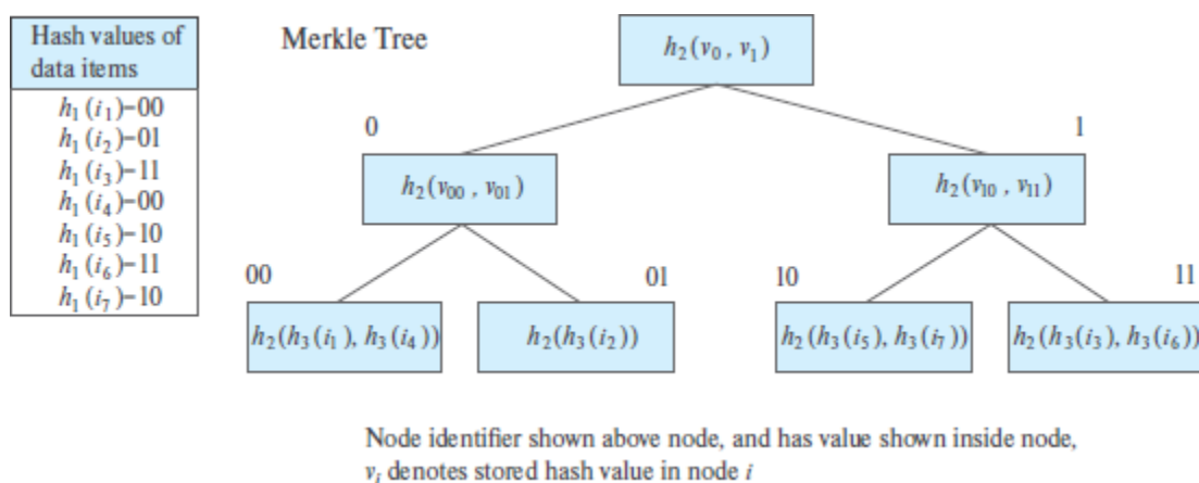
Figure 23.8 Example of Merkle tree.
