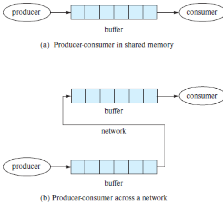
Figure 22.5 Producer and consumer with buffer.
