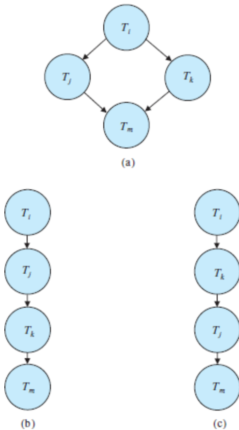
Figure 17.12 Illustration of topological sorting.
