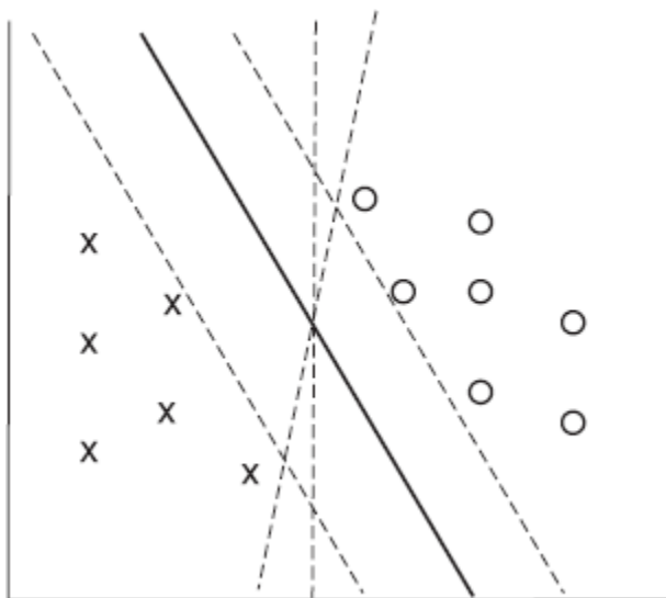
Figure 11.12 Example of a Support Vector Machine classifier.
