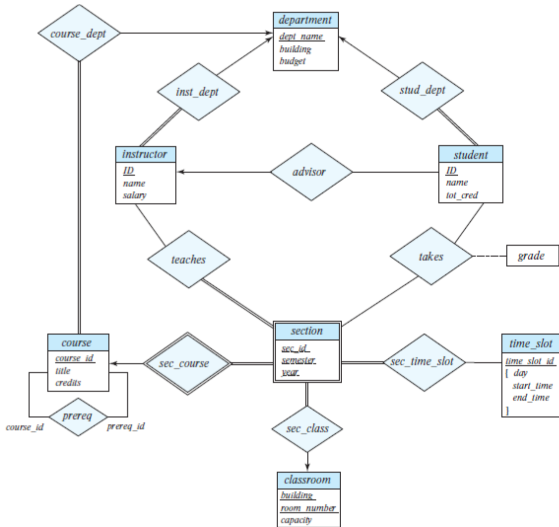
Figure 6.15 E-R diagram for a university enterprise.
