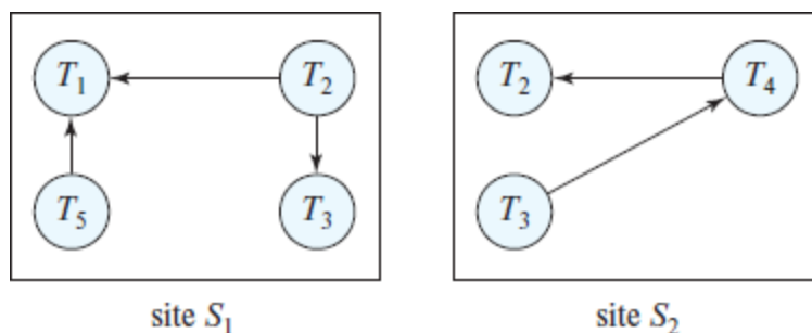
Figure 23.4 Local wait-for graphs.
