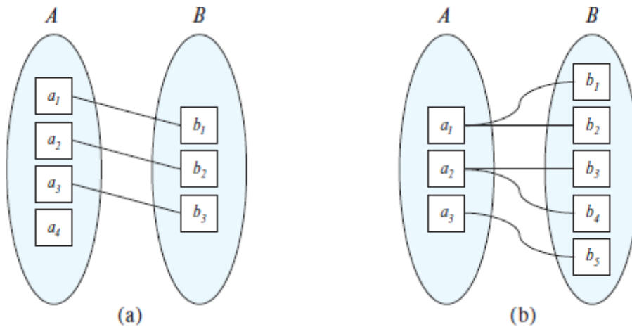
Figure 6.9 Mapping cardinalities. (a) One-to-one. (b) One-to-many.
