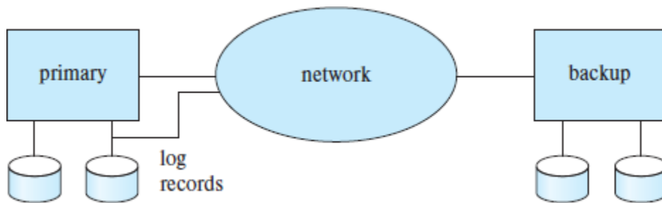
Figure 19.6 Architecture of remote backup system.
