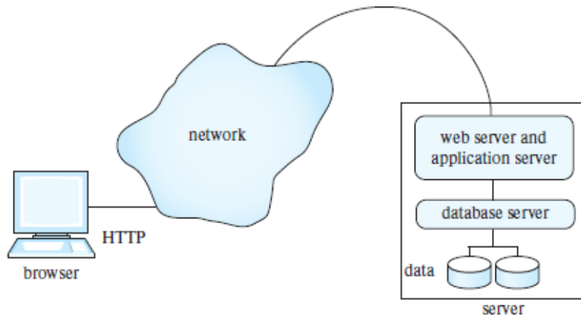
Figure 9.6 Two-layer web application architecture.
