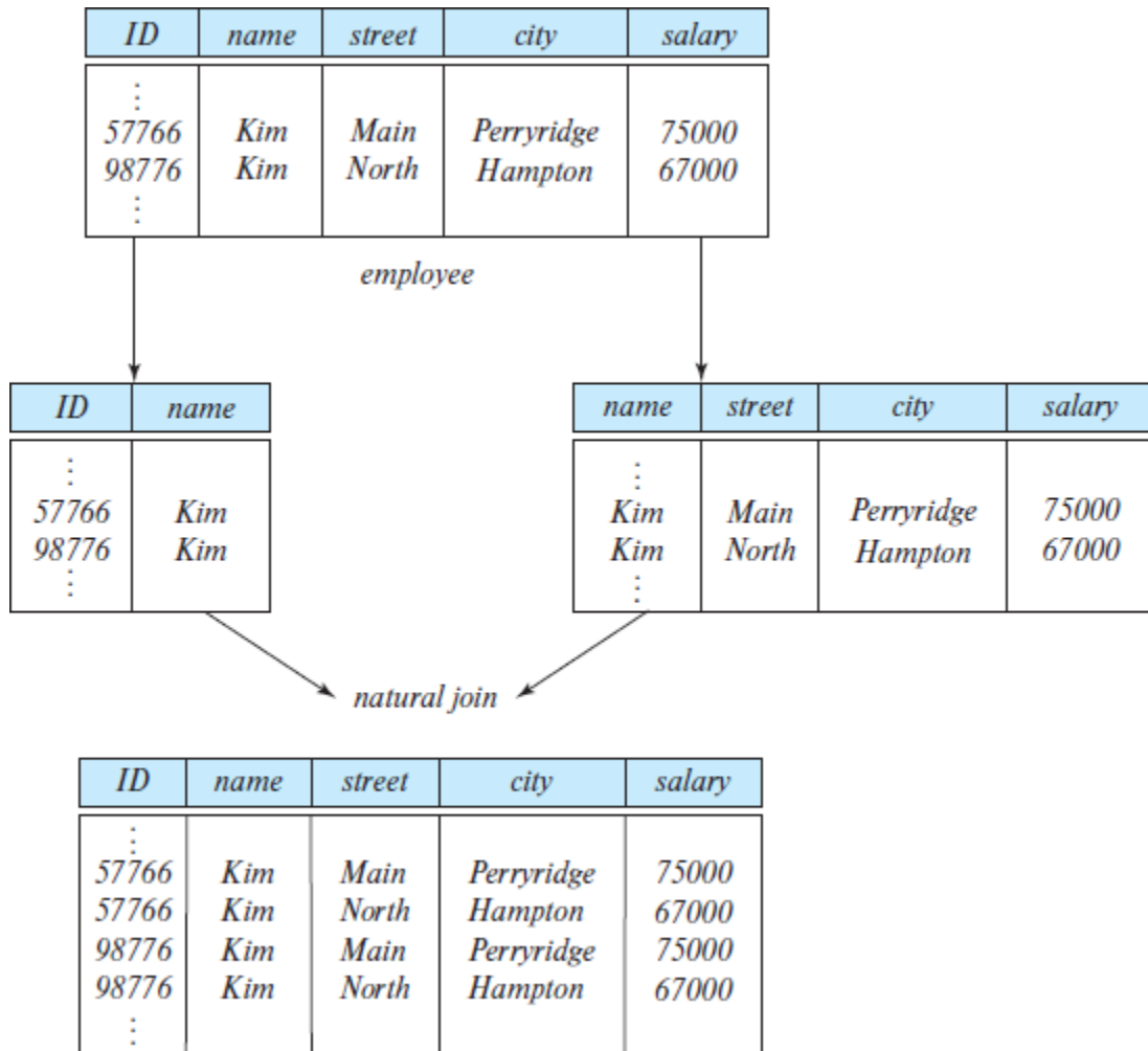
Figure 7.3 Loss of information via a bad decomposition.
