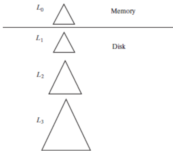
Figure 14.26 Log-structured merge tree with three levels.
