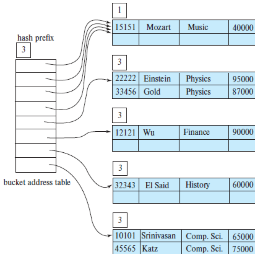
Figure 24.14 Hash structure after seven insertions.
