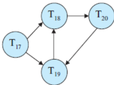
Figure 18.14 Wait-for graph with a cycle.
