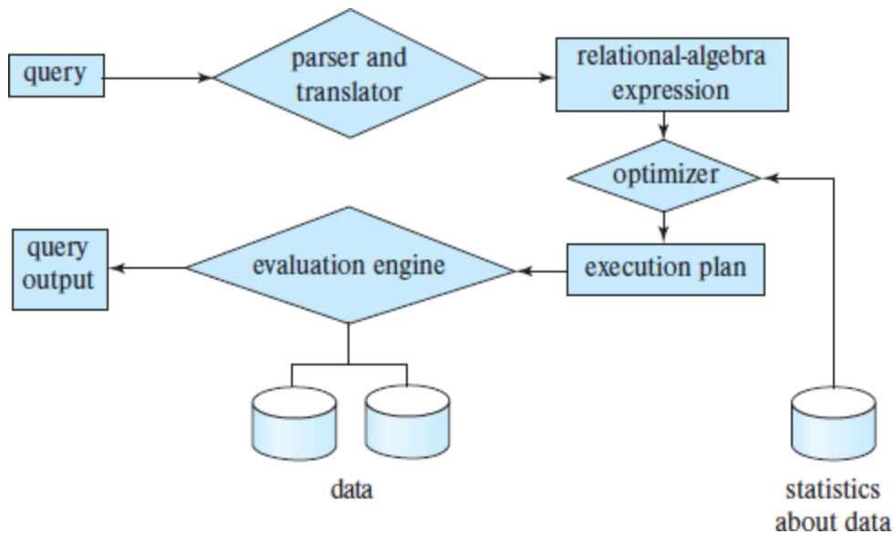
Figure 15.1 Steps in query processing.
