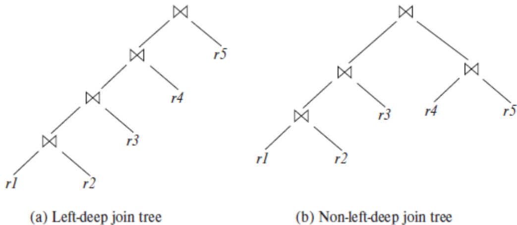
Figure 16.8 Left-deep join trees.
