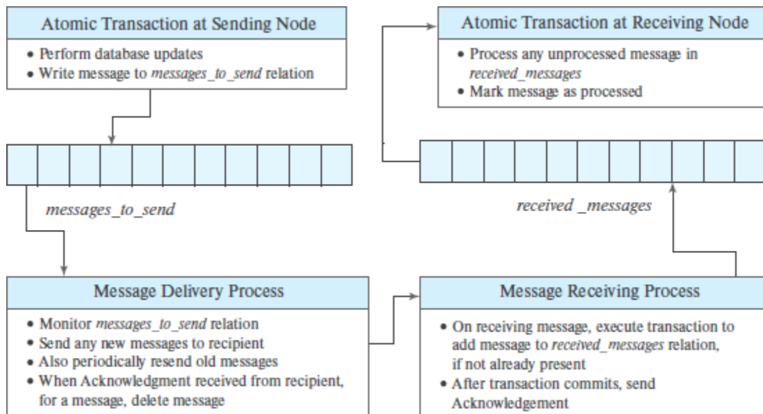
Figure 23.3 Implementation of persistent messaging.
