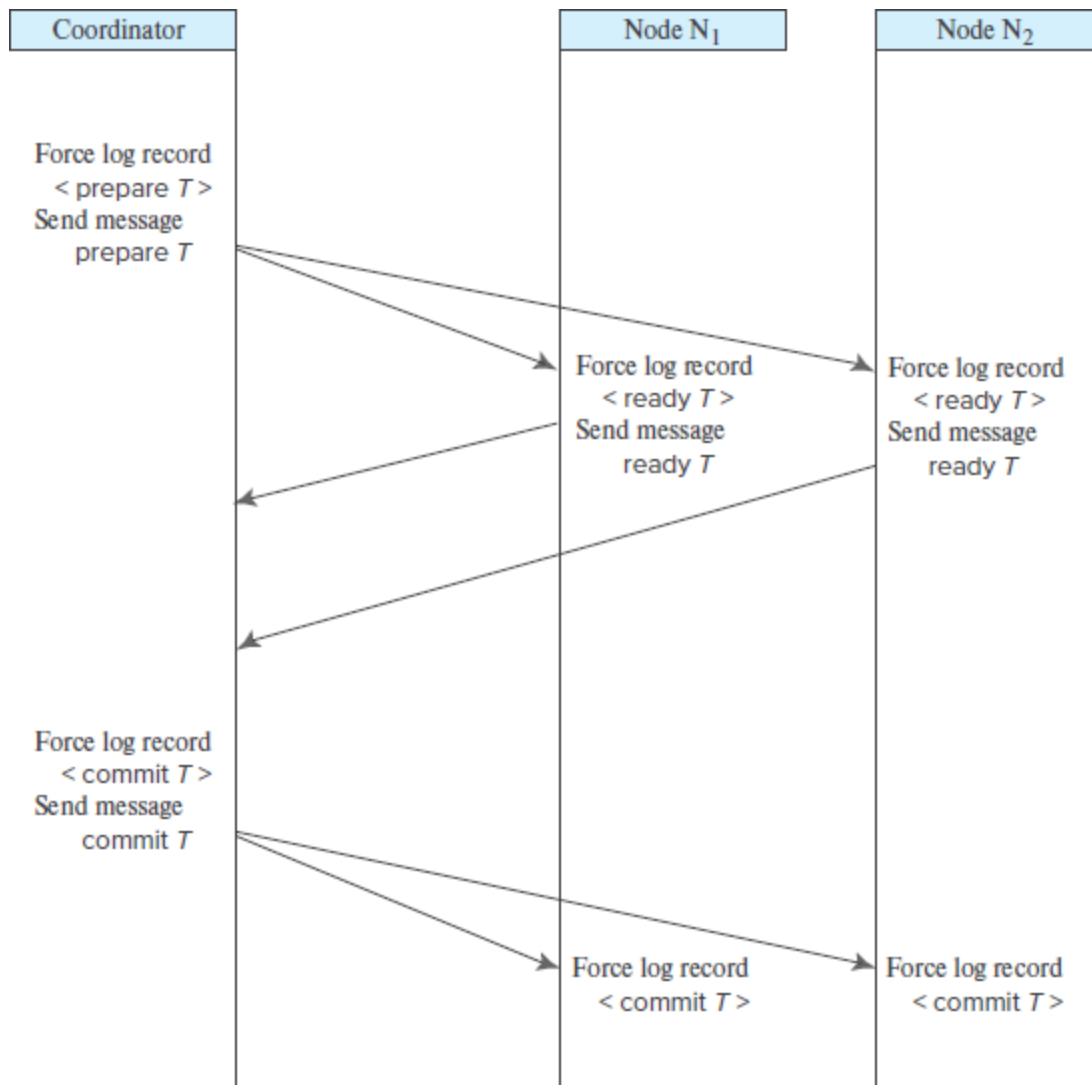
Figure 23.2 Successful execution of 2PC.
