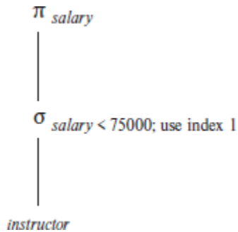
Figure 15.2 A query-evaluation plan.
