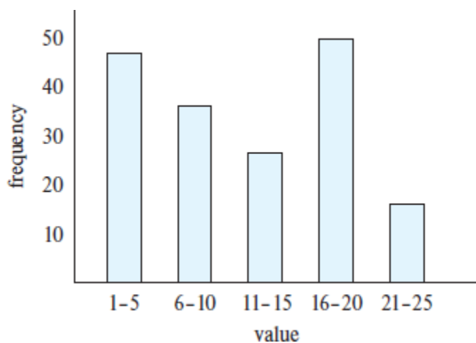
Figure 16.6 Example of histogram.
