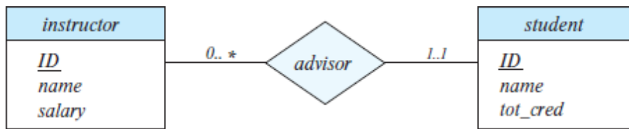
Figure 6.13 Cardinality limits on relationship sets.
