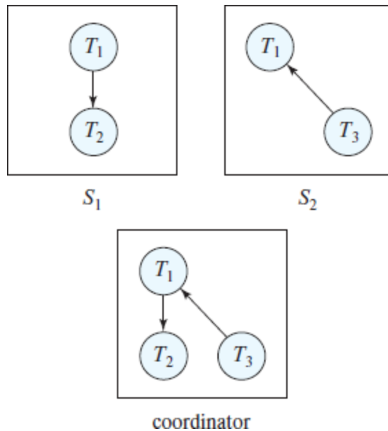
Figure 23.6 False cycles in the global wait-for graph.
