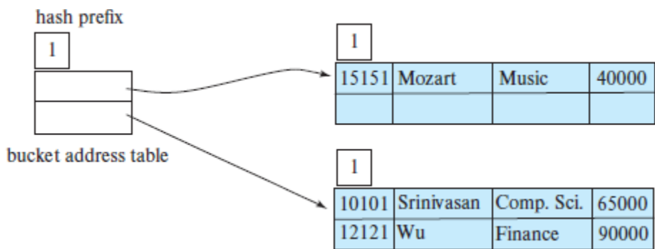
Figure 24.11 Hash structure after three insertions.
