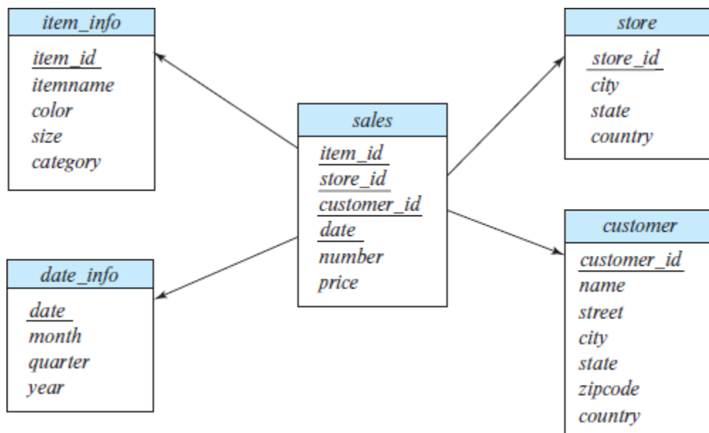
Figure 11.2 Star schema for a data warehouse.
