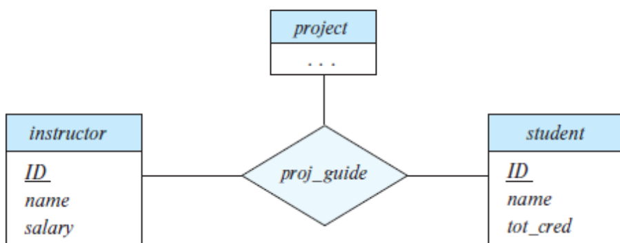
Figure 6.6 E-R diagram with a ternary relationship proj_guide .
