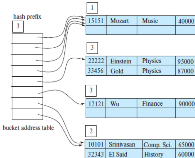
Figure 24.13 Hash structure after six insertions.
