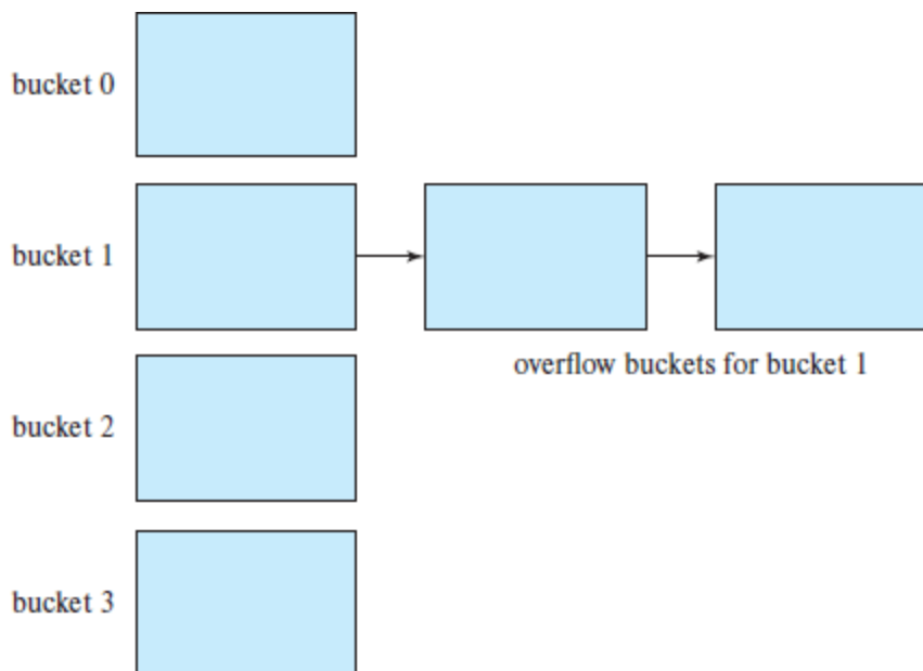
Figure 14.25 Overflow chaining in a disk-based hash structure.
