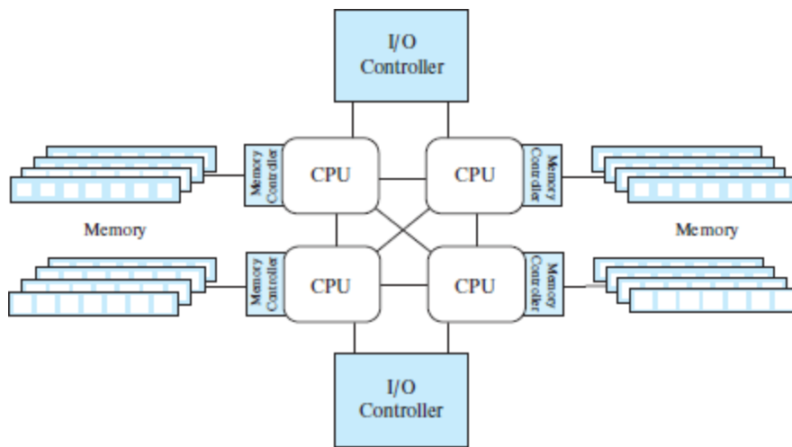
Figure 20.6 Architecture of a modern shared-memory system.
