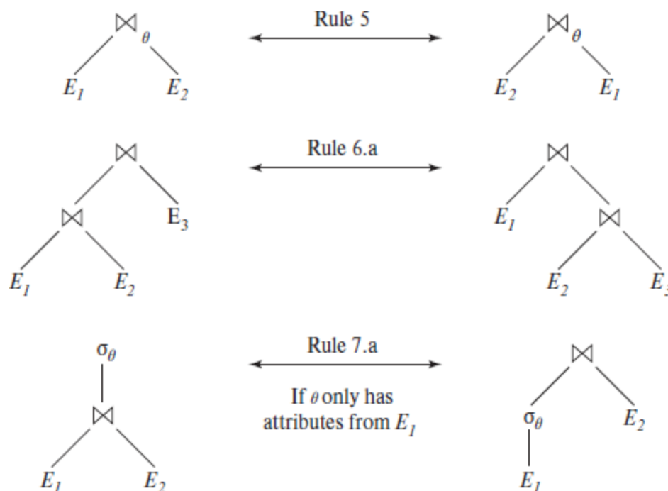
Figure 16.3 Pictorial representation of equivalences.
