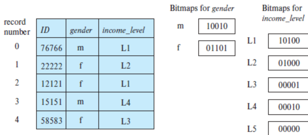
Figure 24.3 Bitmap indices on relation instructor_info .
