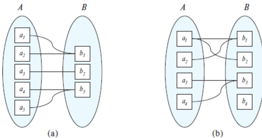
Figure 6.10 Mapping cardinalities. (a) Many-to-one. (b) Many-to-many.
