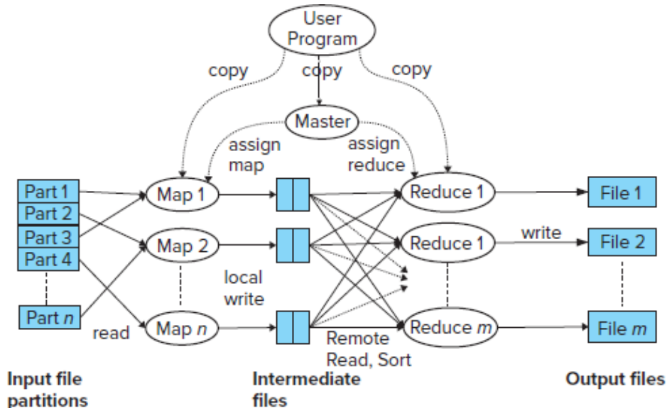
Figure 10.8 Parallel processing of MapReduce job.
