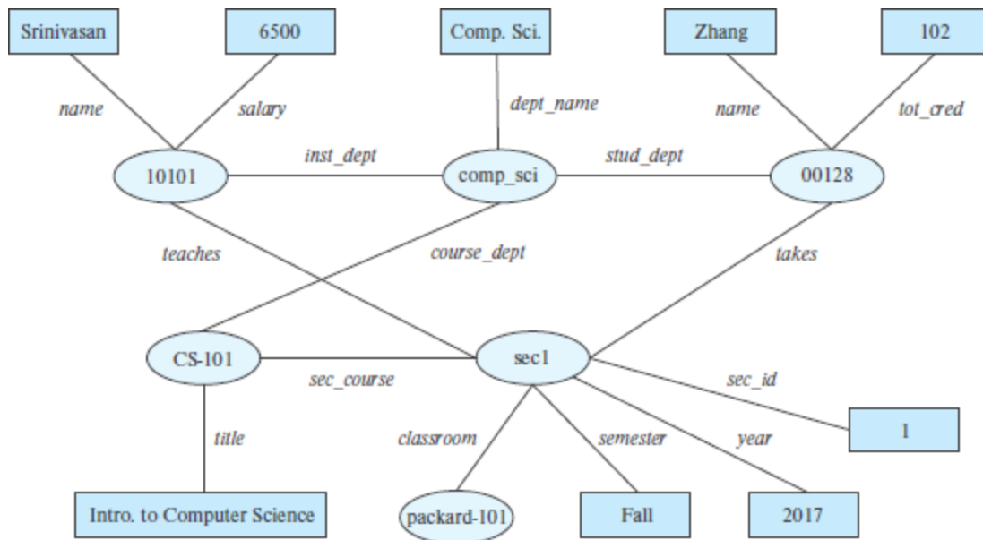
Figure 8.4 Graph representation of RDF data.
