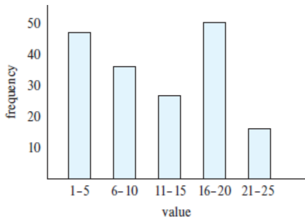
Figure 21.2 Example of histogram.
