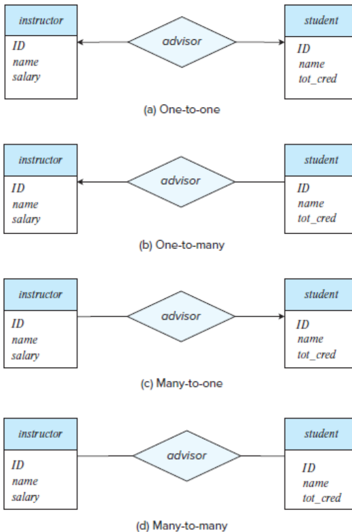
Figure 6.11 Relationship cardinalities.
