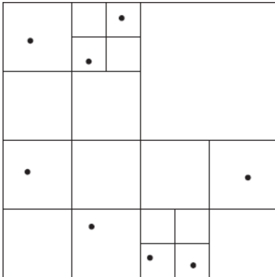
Figure 24.4 Division of space by a quadtree.
