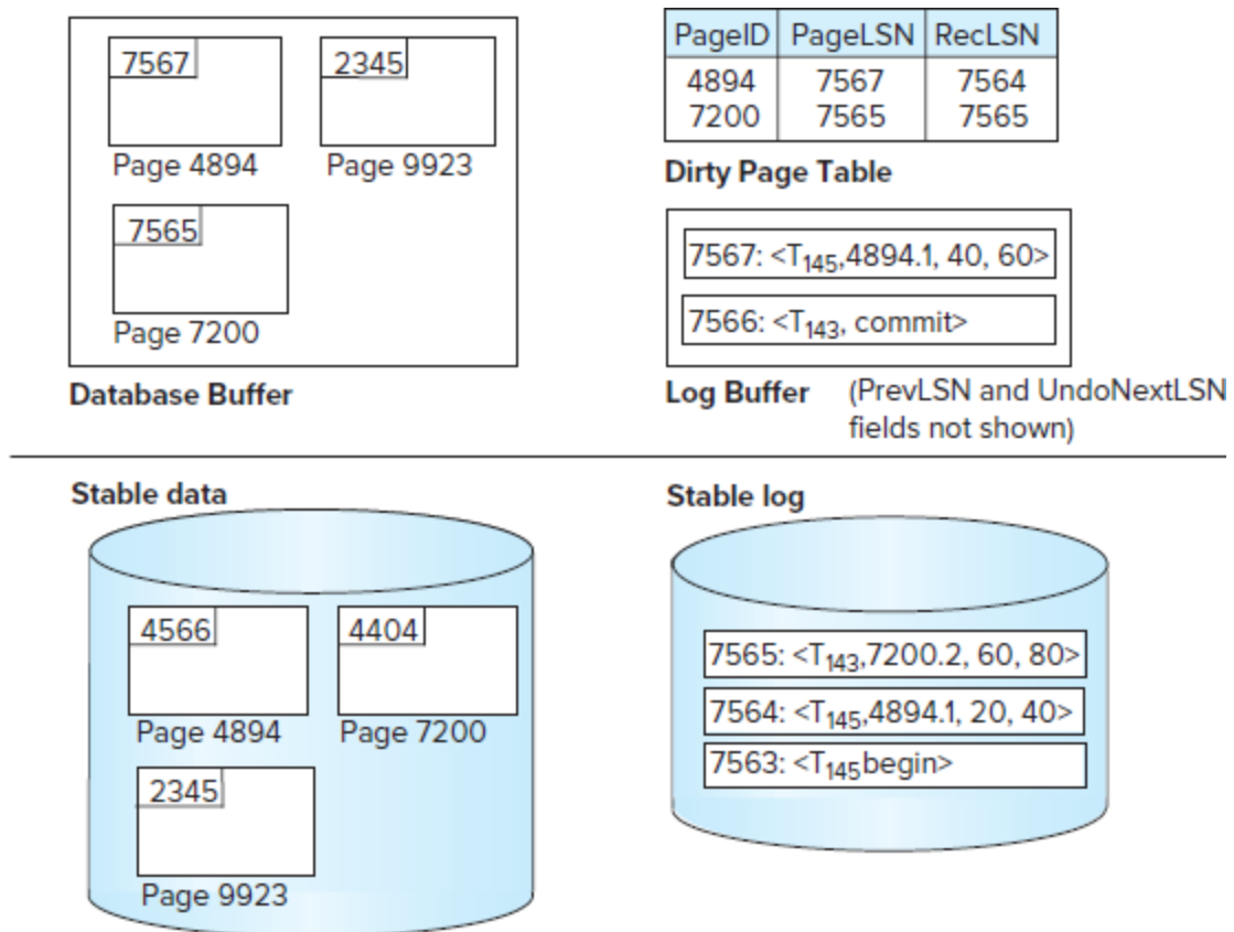
Figure 19.9 Data structures used in ARIES.
