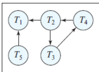
Figure 23.5 Global wait-for graph for Figure 23.4 .
