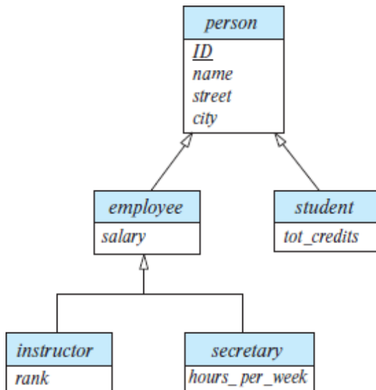
Figure 6.18 Specialization and generalization.
