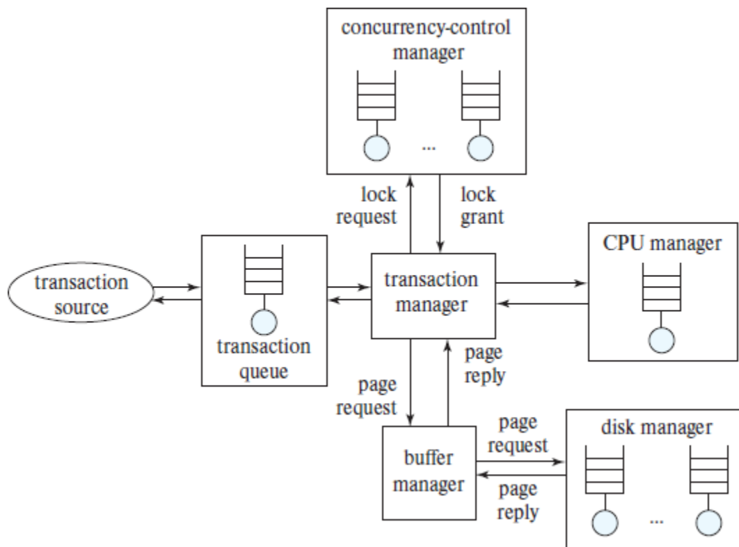
Figure 25.1 Queues in a database system.
