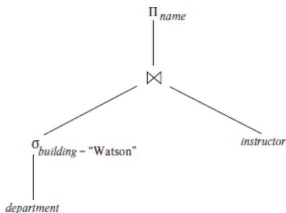
Figure 15.11 Pictorial representation of an expression.
