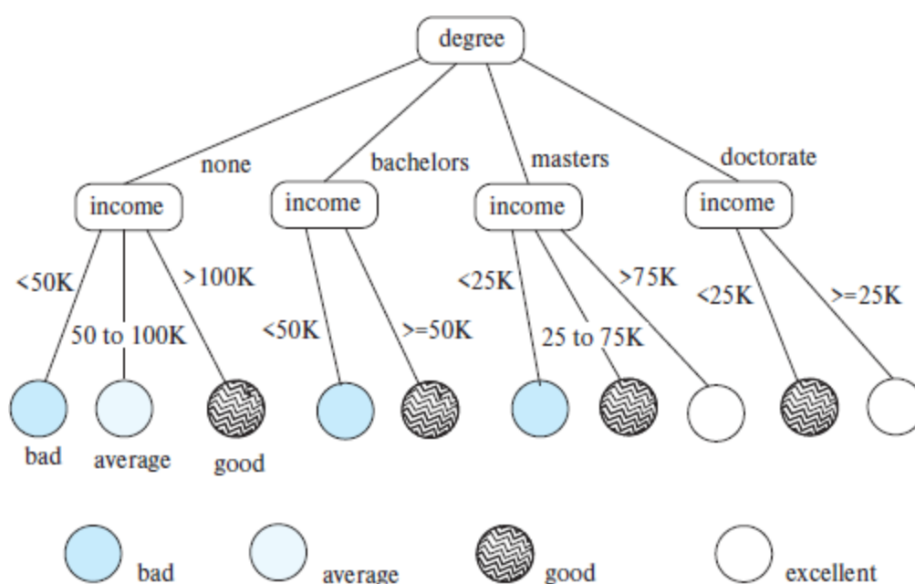
Figure 11.11 Classification tree.
