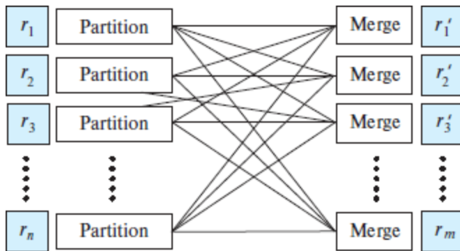
Figure 22.6 The exchange operator used for repartitioning.
