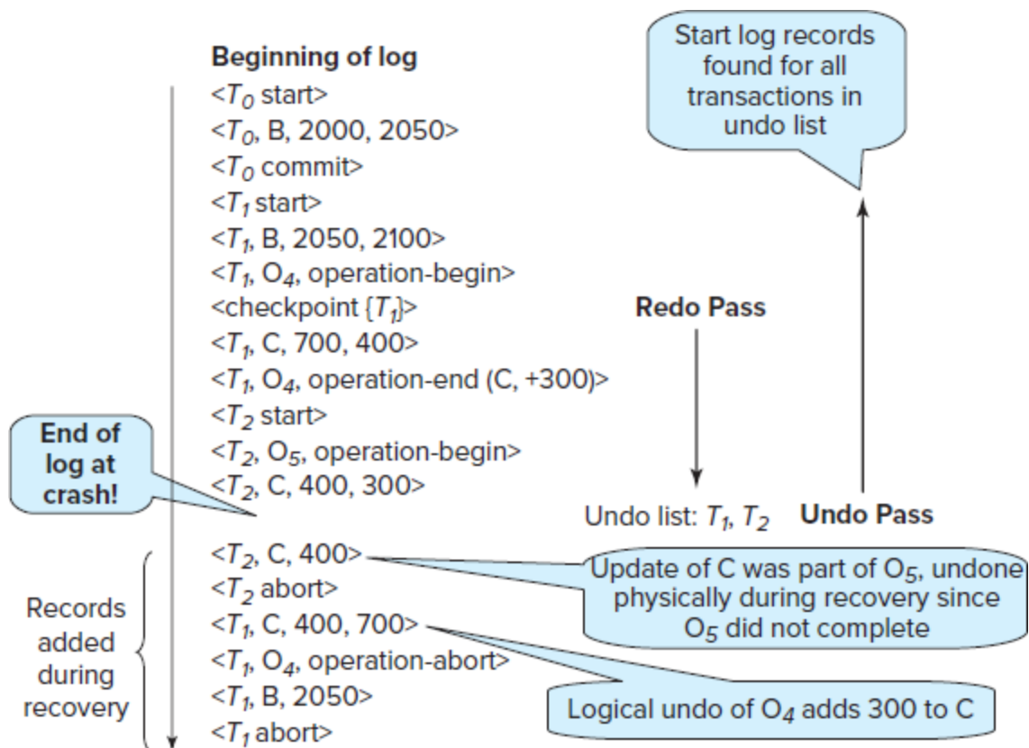
Figure 19.8 Failure recovery actions with logical undo operations.
