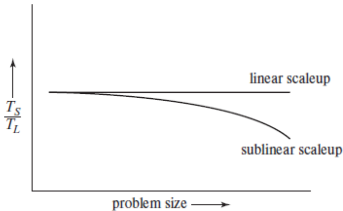
Figure 20.3 Scaleup with increasing problem size and resources.
