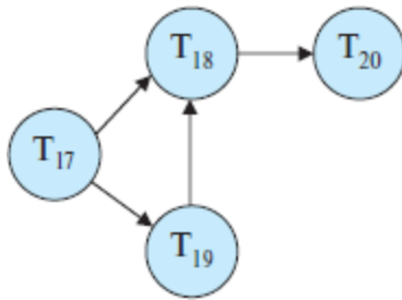
Figure 18.13 Wait-for graph with no cycle.
