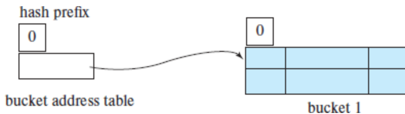
Figure 24.10 Initial extendable hash structure.
