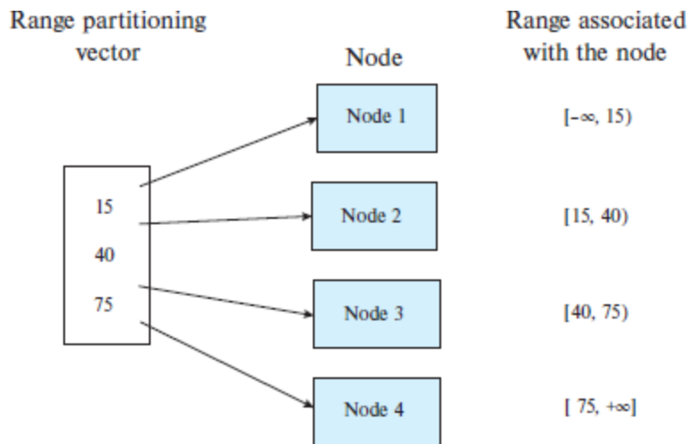
Figure 21.1 Example of range partitioning vector.
