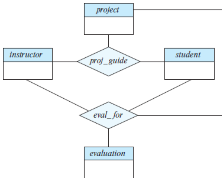
Figure 6.19 E-R diagram with redundant relationships.
