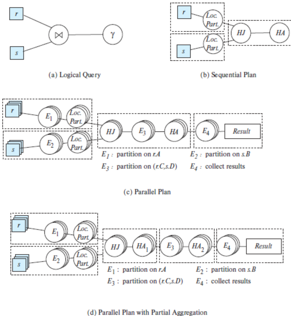
Figure 22.7 Parallel query execution plans.
