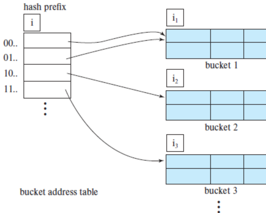
Figure 24.8 General extendable hash structure.
