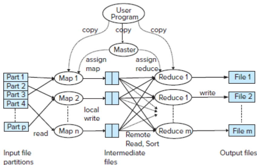
Figure 22.4 Parallel processing of MapReduce job.
