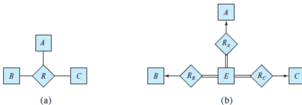
Figure 6.25 Ternary relationship versus three binary relationships.
