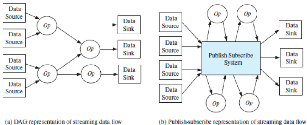
Figure 10.11 Routing of streams using DAG and publish-subscribe representations.
