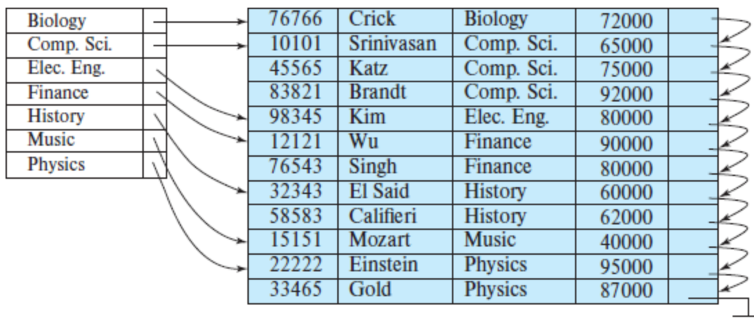
Figure 14.4 Dense index with search key dept_name .
