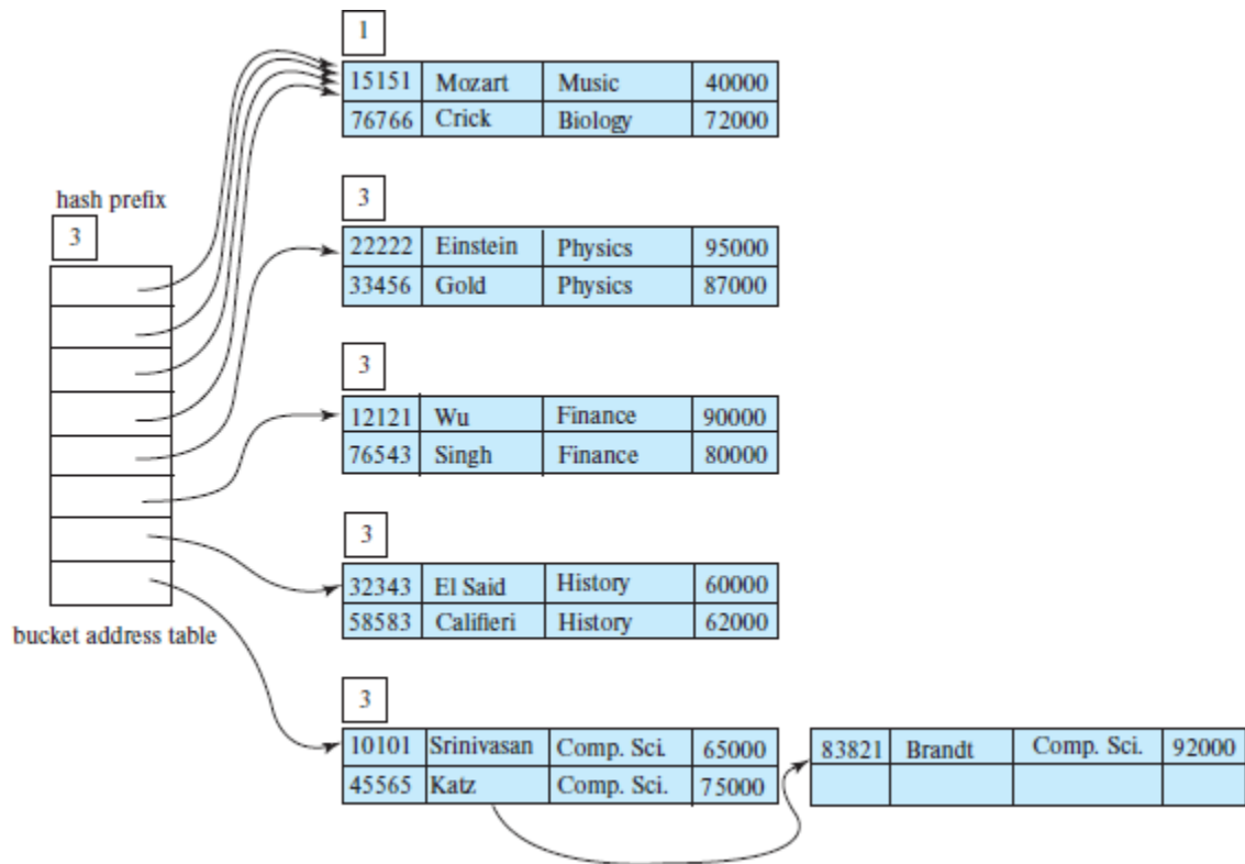
Figure 24.15 Hash structure after 11 insertions.
