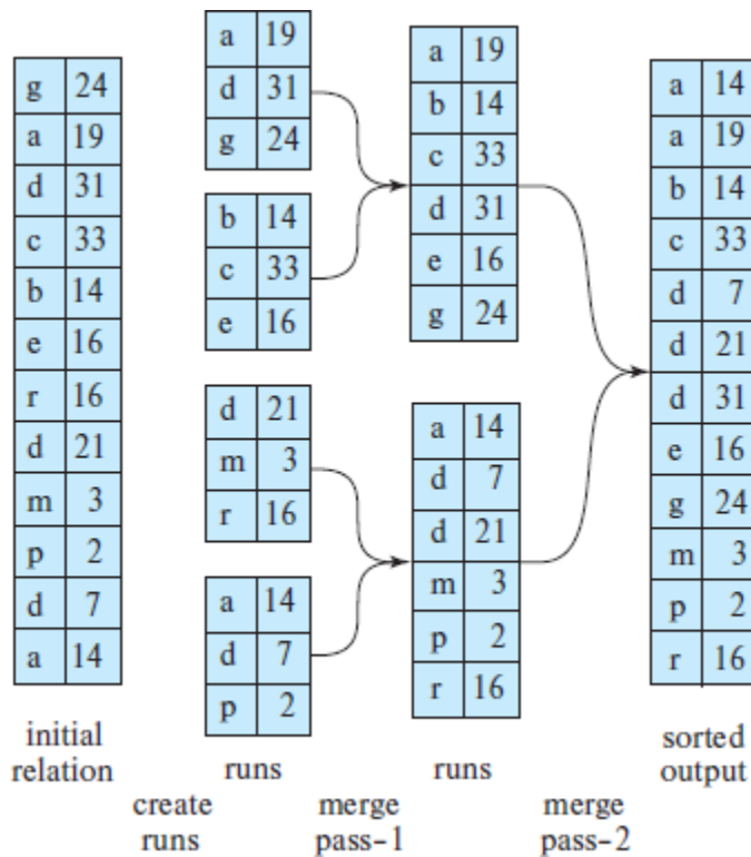
Figure 15.4 External sorting using sort-merge.
