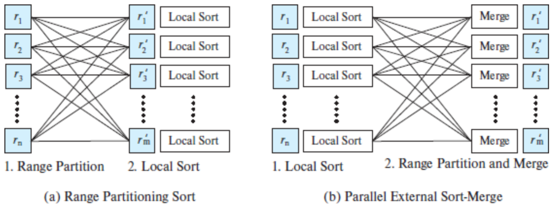
Figure 22.1 Parallel sorting algorithms.
