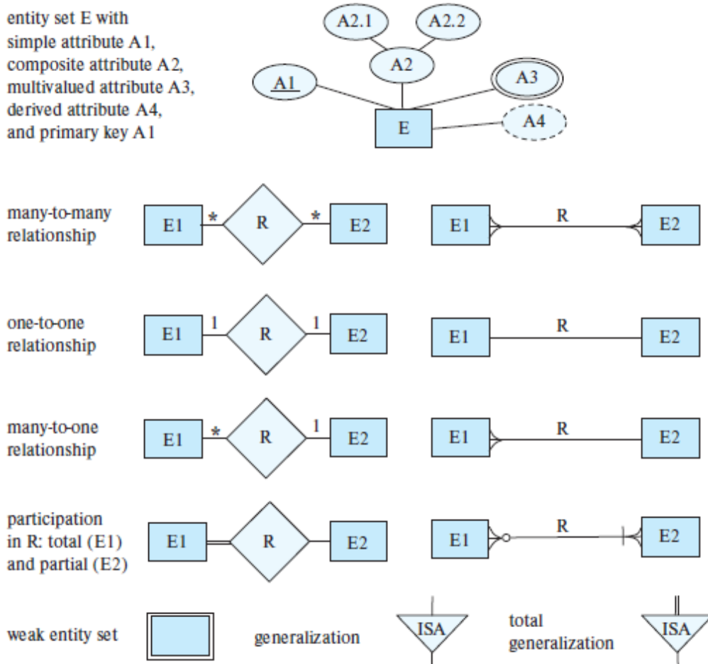
Figure 6.27 Alternative E-R notations.
