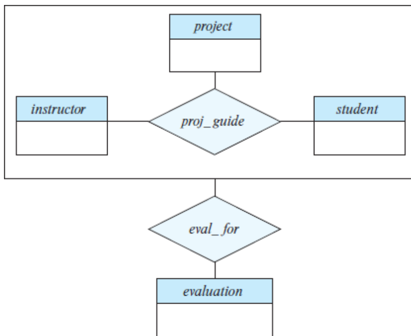
Figure 6.20 E-R diagram with aggregation.
