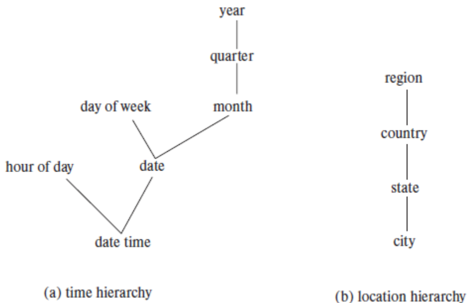
Figure 11.6 Hierarchies on dimensions.
