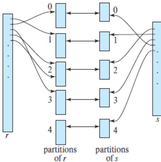
Figure 15.9 Hash partitioning of relations.
