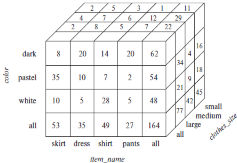
Figure 11.5 Three-dimensional data cube.
