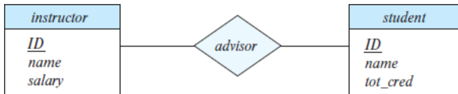
Figure 6.3 E-R diagram showing relationship set advisor .
