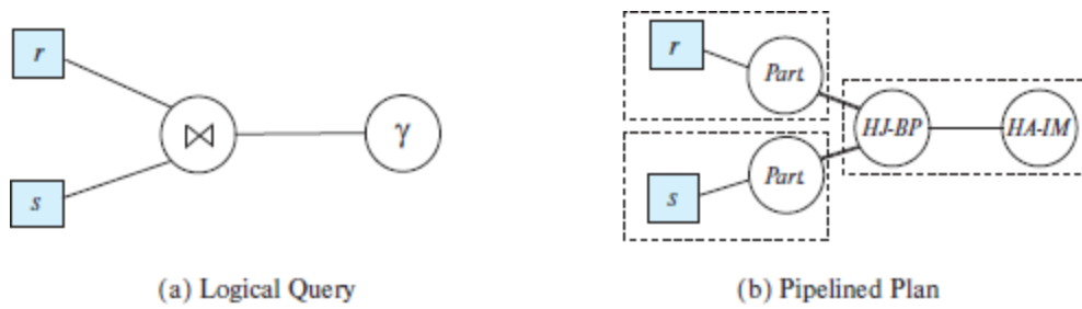
Figure 15.12 Query plan with pipelining.
