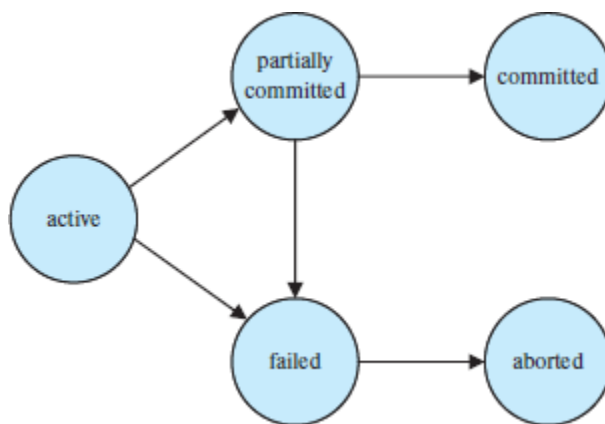
Figure 17.1 State diagram of a transaction.
