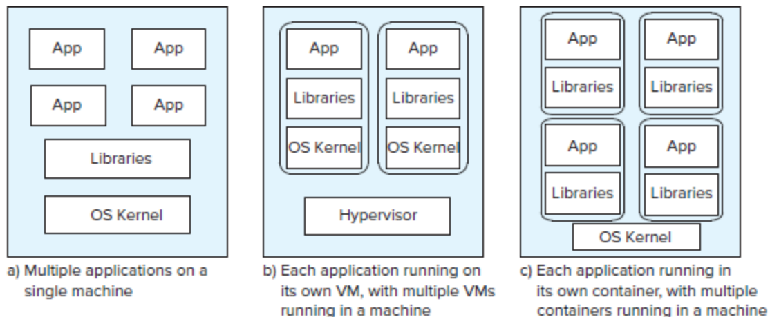
Figure 20.11 Application deployment alternatives.
