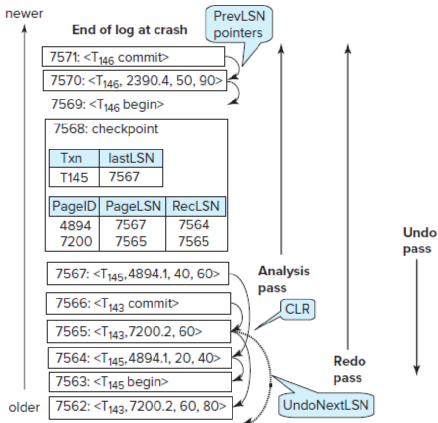
Figure 19.10 Recovery actions in ARIES.
