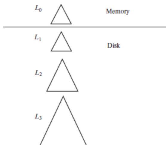
Figure 24.1 Log-structured merge tree with three levels.
