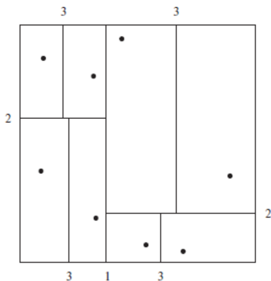
Figure 14.29 Division of space by a k-d tree.
