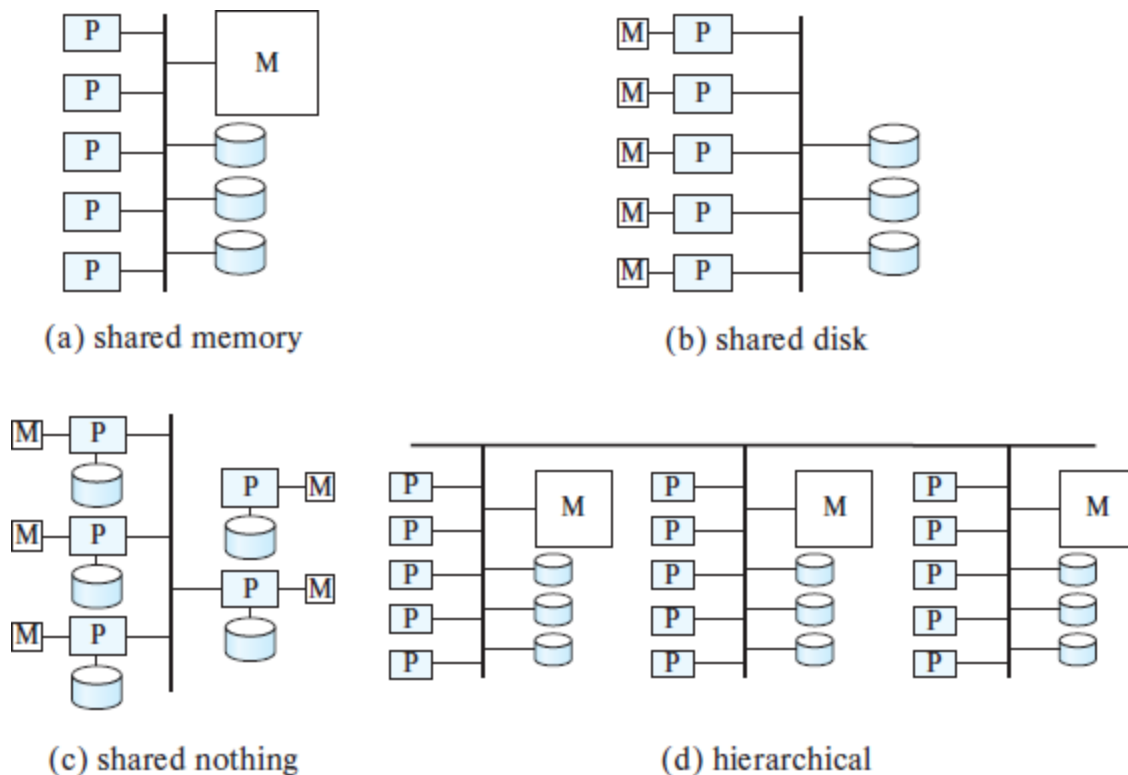
Figure 20.5 Parallel database architectures.
