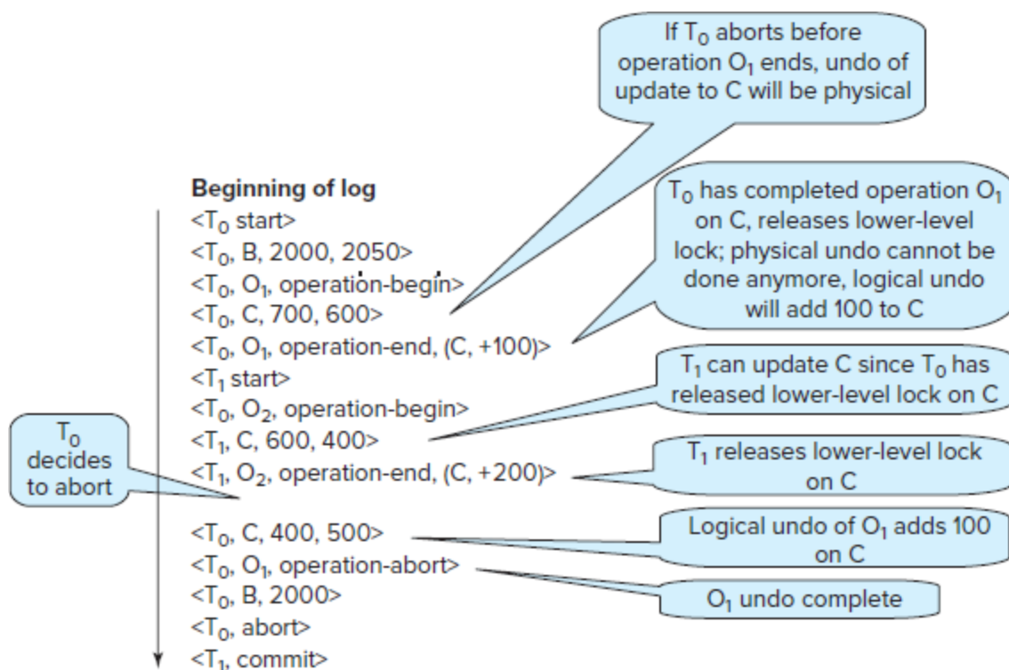
Figure 19.7 Transaction rollback with logical undo operations.
