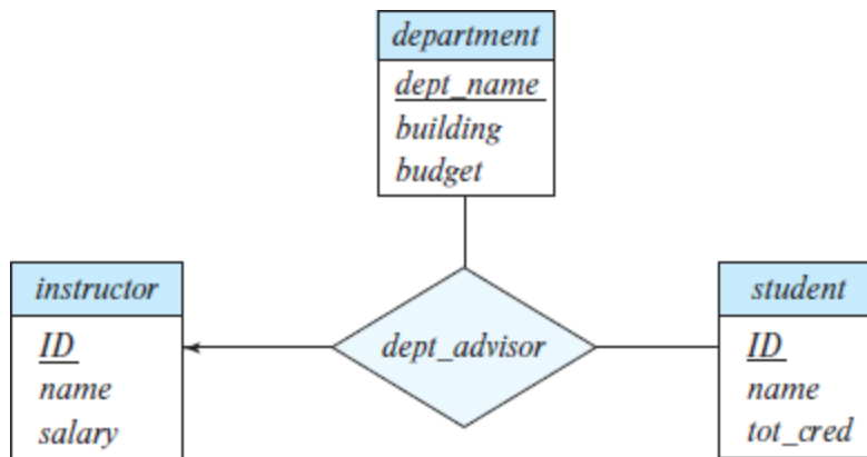
Figure 7.6 The dept_advisor relationship set.
