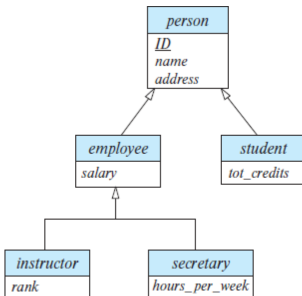
Figure 8.9 Specialization and generalization.
