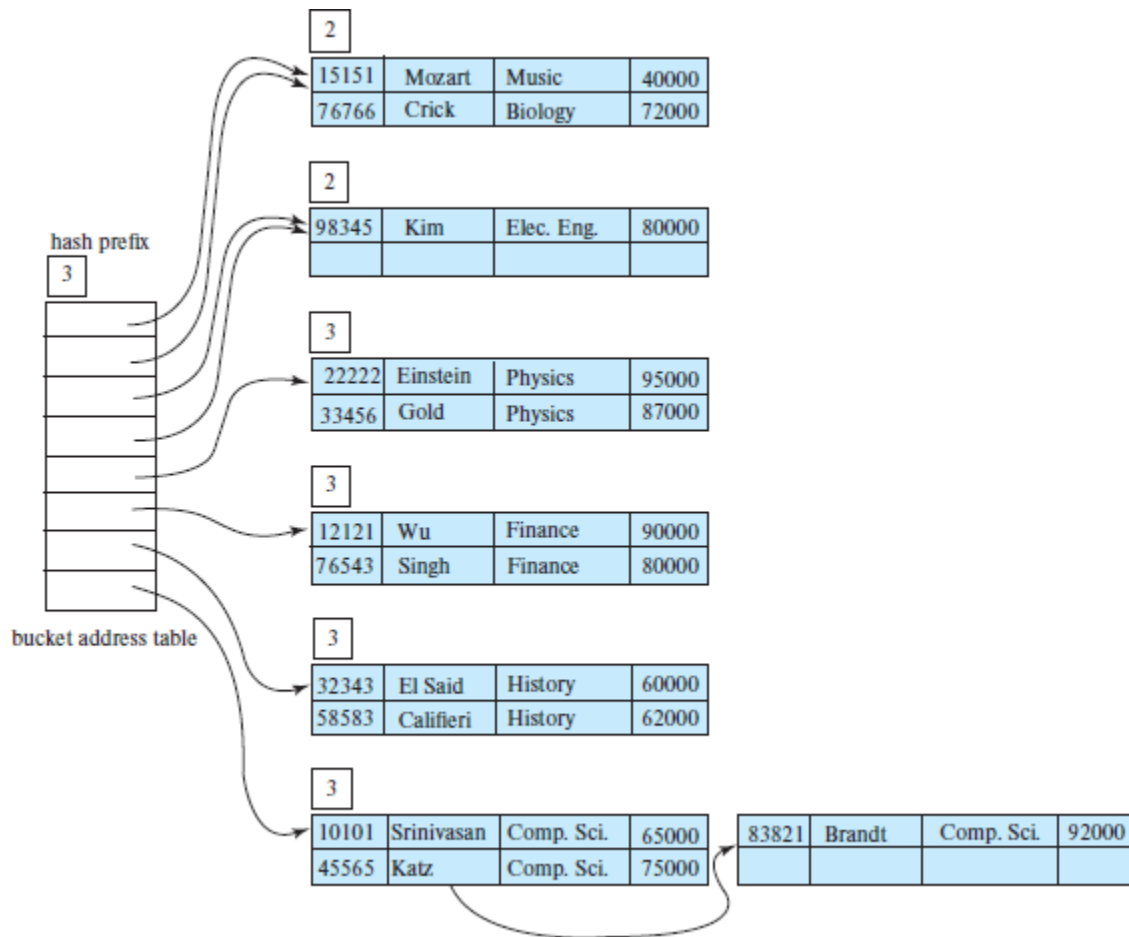
Figure 24.16 Extendable hash structure for the instructor file.
