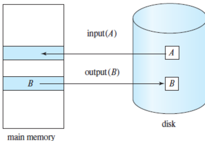
Figure 19.1 Block storage operations.
