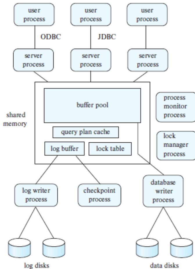
Figure 20.1 Shared memory and process structure.
