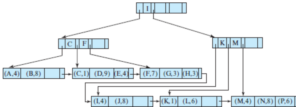
Figure 14.22 B + -tree file organization.
